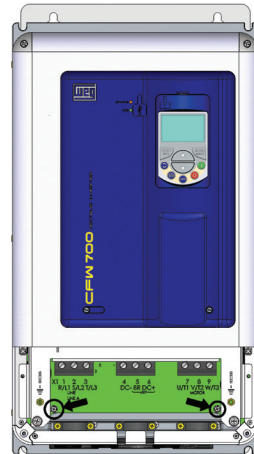
Inverter without the bottom front cover Convertidor sin la tapa frontal inferior Inversor sem a tampa frontal inferior
